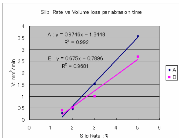
Slip Ratio VS Wear Volume
