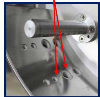
Turret Section
